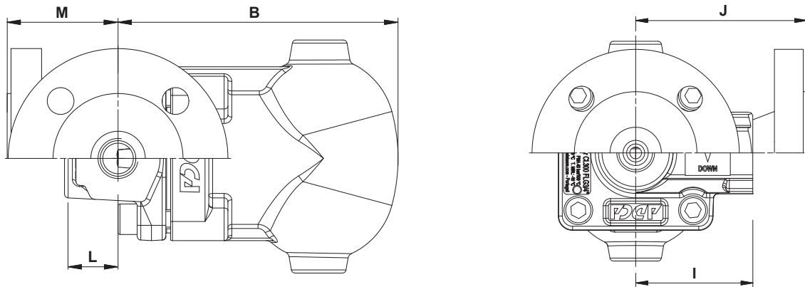
Angled design
