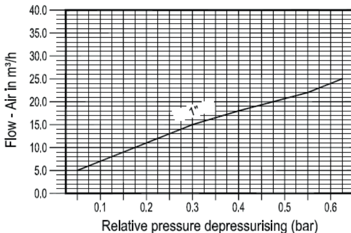
CAPACITY CHART
