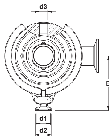
Optional pressure gauge connections.
