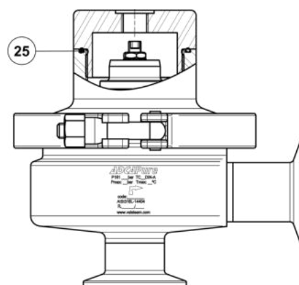
Dome-loaded top
